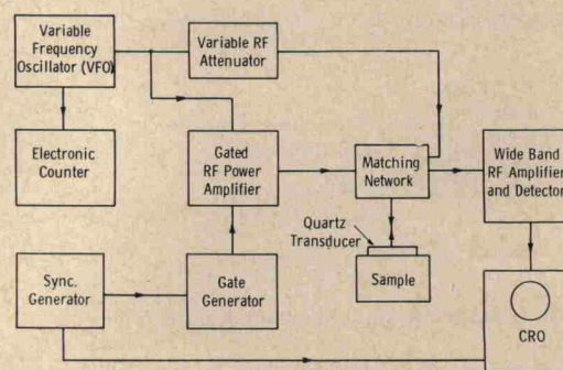
FIG. 4. Block diagram of pulse/cw system.
